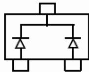
BAV70:A4
