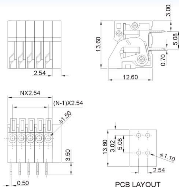
DG141R-2.54
