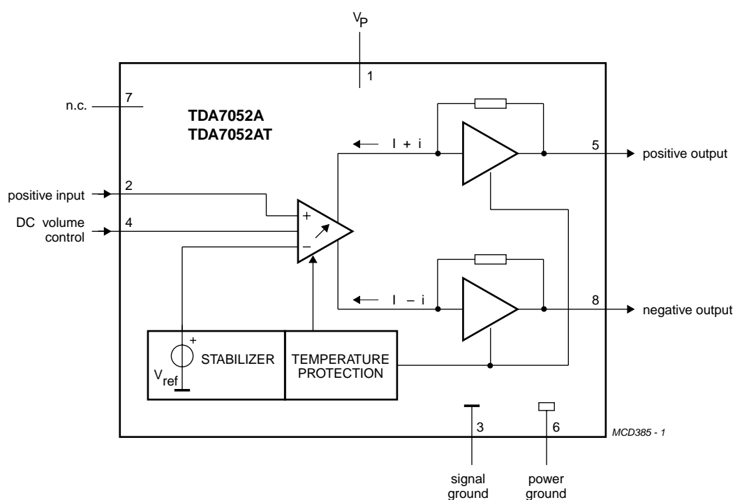
Fig.1 Block diagram.
