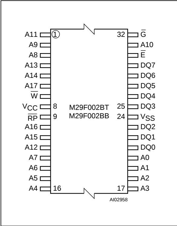
Figure 3. TSOP Connections
